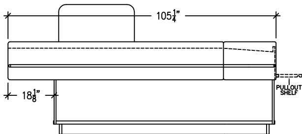
E3 01 OUTSIDE ELEVATION: SB-230 LEFTHAND CHECK STAND SCALE: 3/8" = 1'-0"
