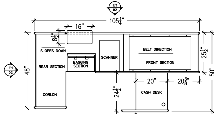
P1 01 PLAN VIEW: SB-230 LEFTHAND CHECK STAND SCALE: 3/8" = 1'-0"
