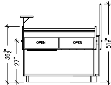
E1 01 END ELEVATION: SB-230 LEFTHAND CHECK STAND SCALE: 3/8" = 1'-0"
