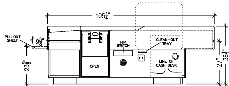
E2 01 INSIDE ELEVATION: SB-230 LEFTHAND CHECK STAND SCALE: 3/8" = 1'-0"
