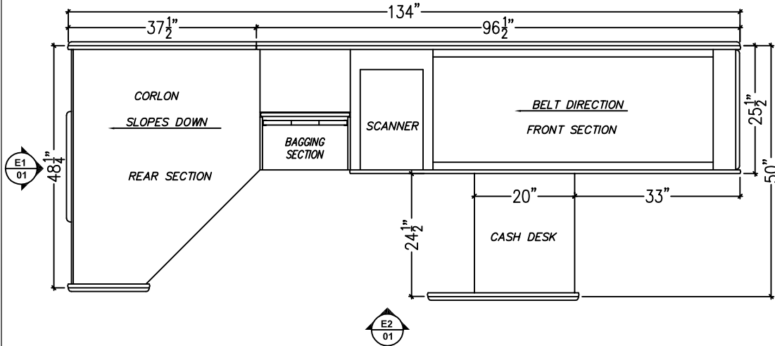
P1 01 PLAN VIEW: SB-215 CHECKOUT LEFT HAND SHOWN SCALE: 3/8" = 1'-0"
