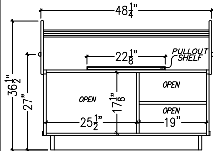
E1 01 END ELEVATION: SB-215 CHECKOUT L/H SHOWN SCALE: 3/8" = 1'-0"
