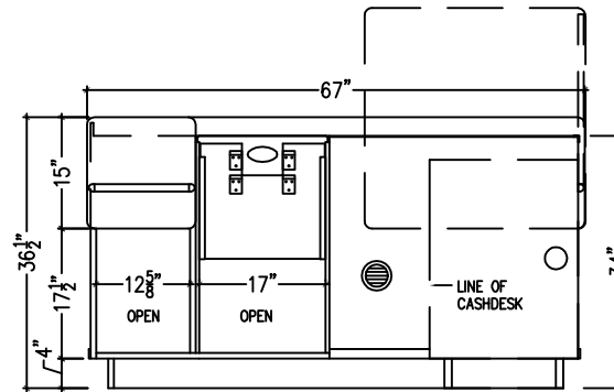
E2 INSIDE ELEVATION: SB-142 CHECKOUT L/H SHOWN SCALE: 3/8" = 1'-0"
