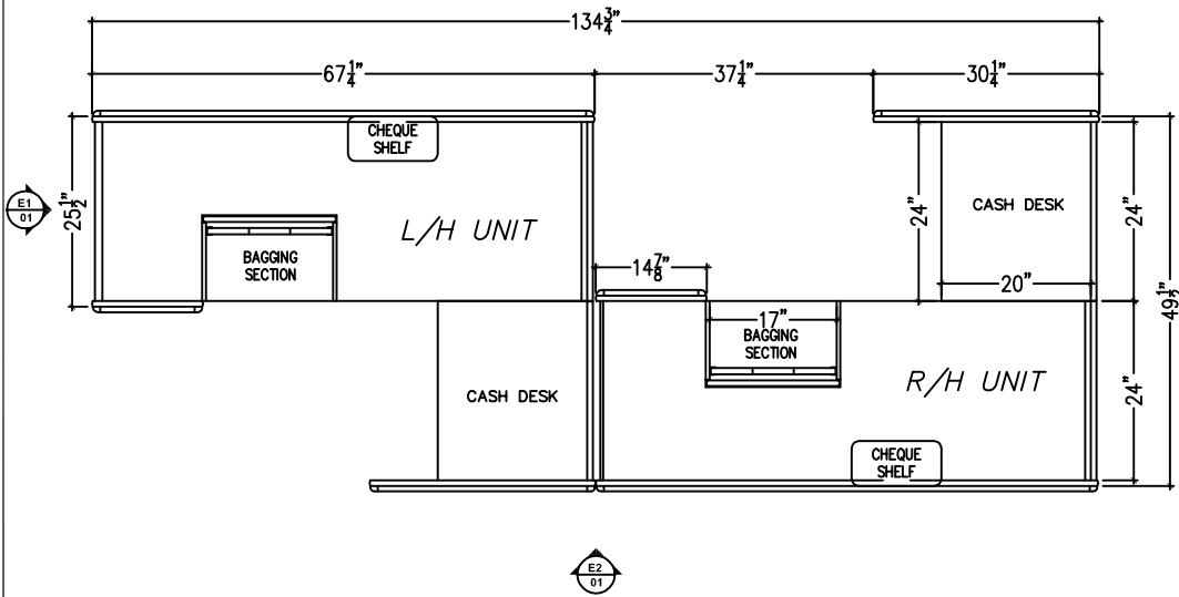
P1 PLAN VIEW: SB-142 CHECKOUT L/H AND R/H SHOWN SCALE: 3/8" = 1'-0"
