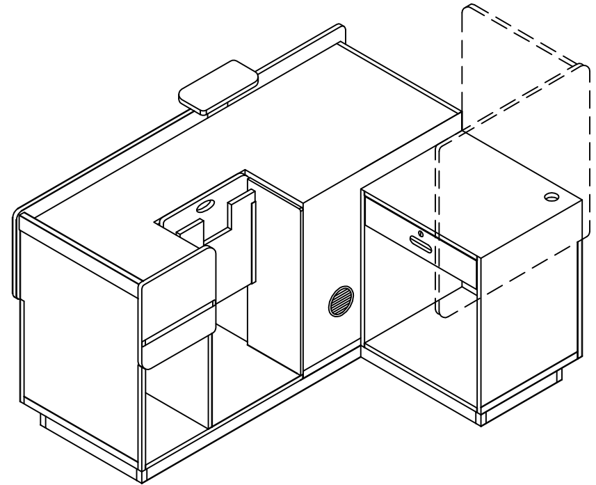
I1 ISOMETRIC VIEW: SB-142 CHECKOUT L/H SHOWN SCALE: NOT TO SCALE
